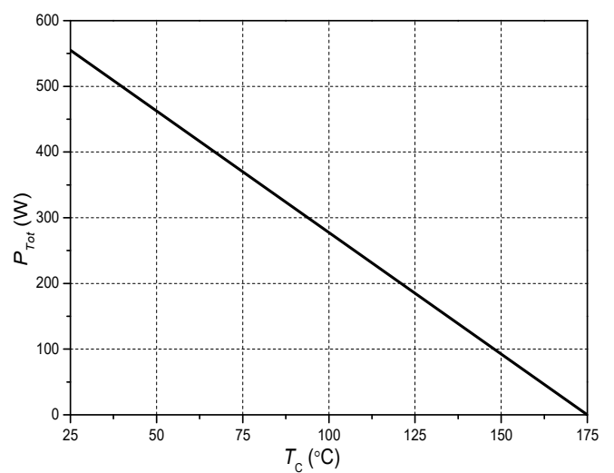
Figure 6. Power Derating
