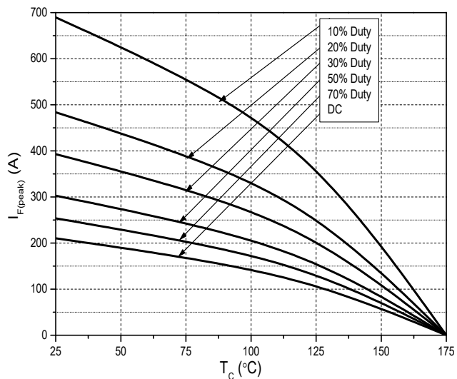
Figure 7. Current Derating
