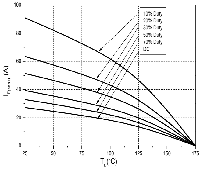
Figure 7. Current Derating
