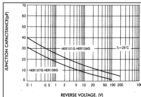
FIG.6-TYPICAL JUNCTION CAPACITANCE
