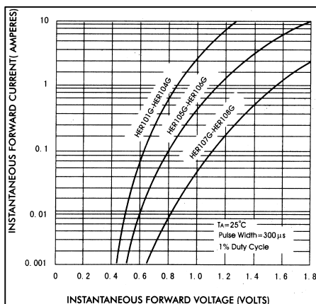
FIG.3-TYPICAL FORWARD CHARACTERISTICS
